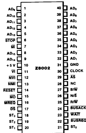
Figure 11a. 40-pin Dual-In-Line Package (DIP), Pin Assignments
