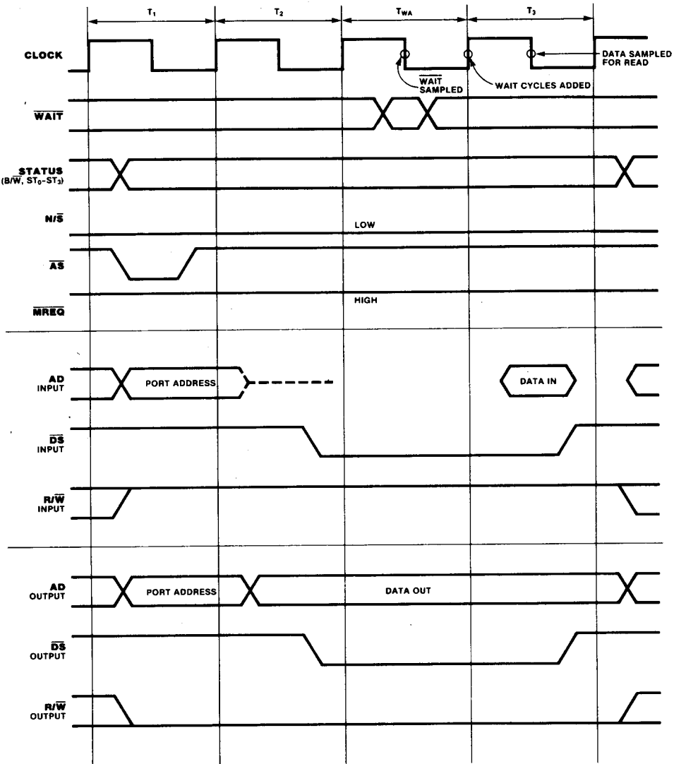
Figure 13. Input/Output Timing
