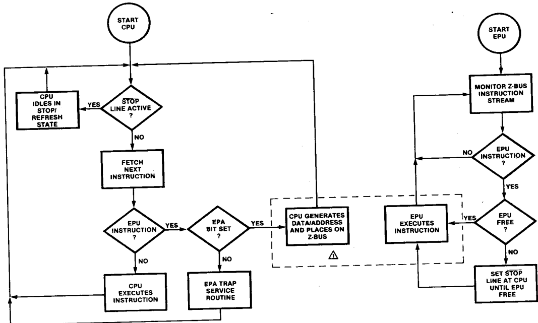
Figure 8. EPA and Z8000 CPU Instruction Execution
