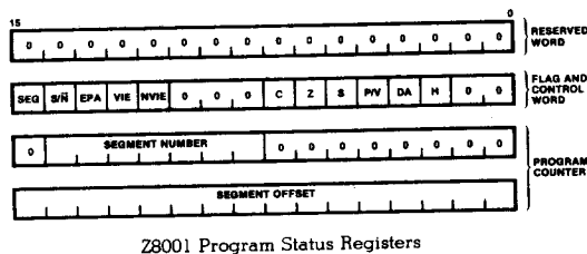
Z8001 Program Status Registers
