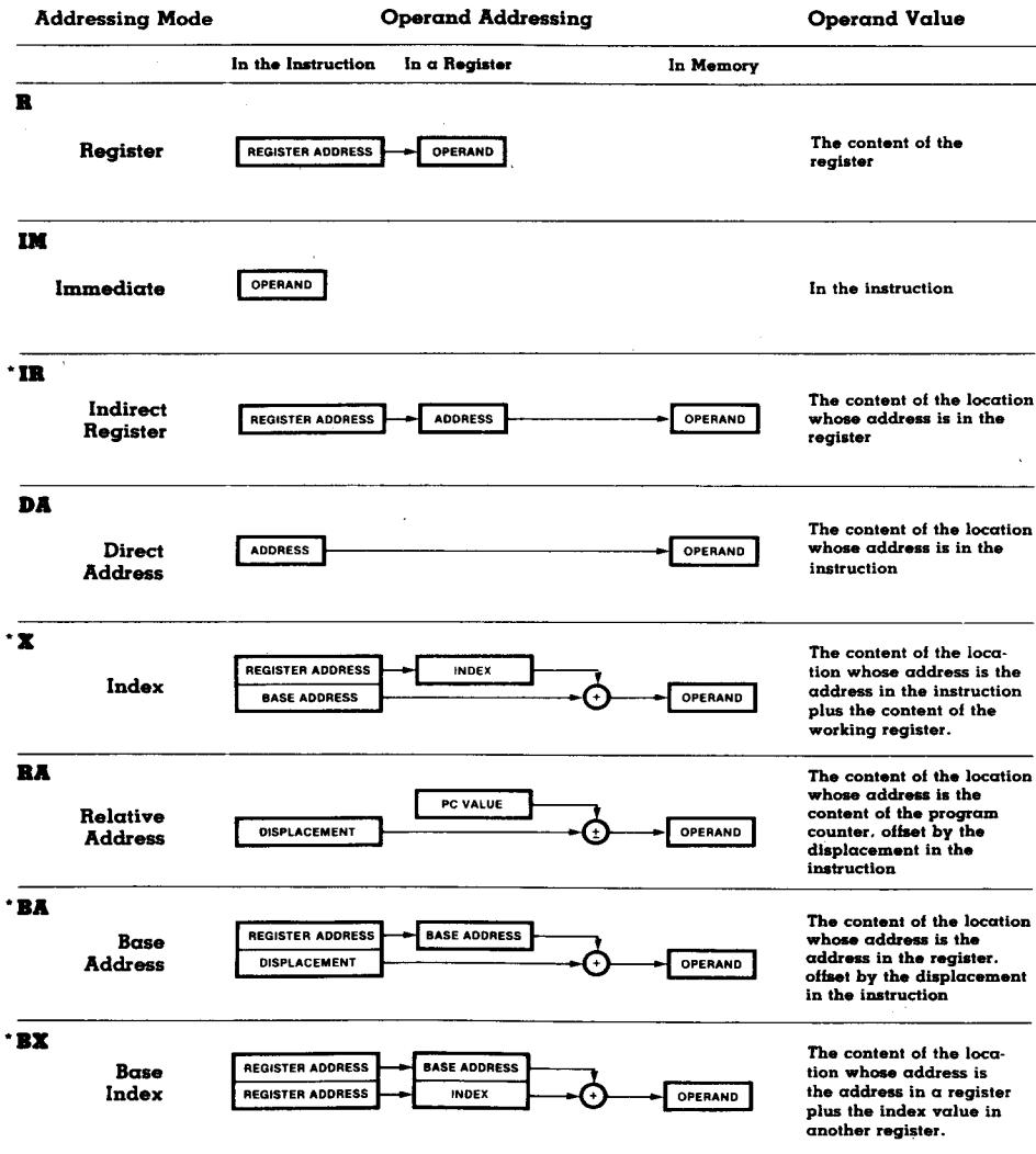
Figure 9. Addressing Modes
