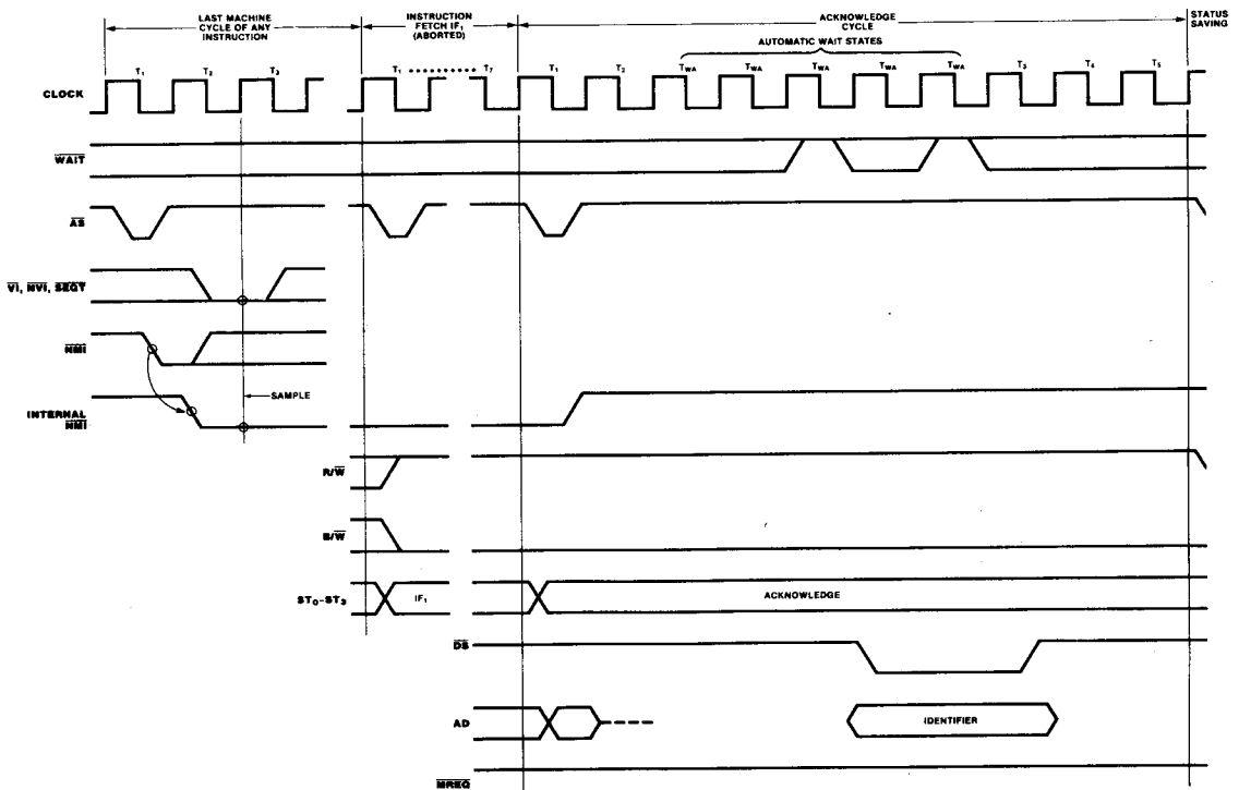
Figure 14. Interrupt and Segment Trap Request/Acknowledge Timing
