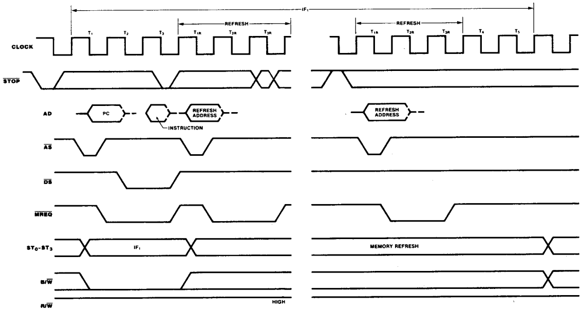
Figure 16. Stop Timing
