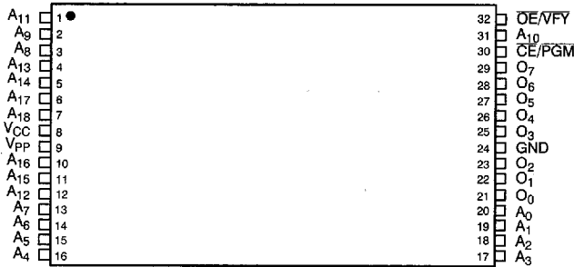
TSOP Top View
