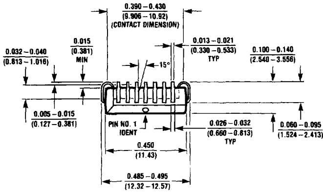
32-Lead PLCC Package Order Number NMC27C010V
