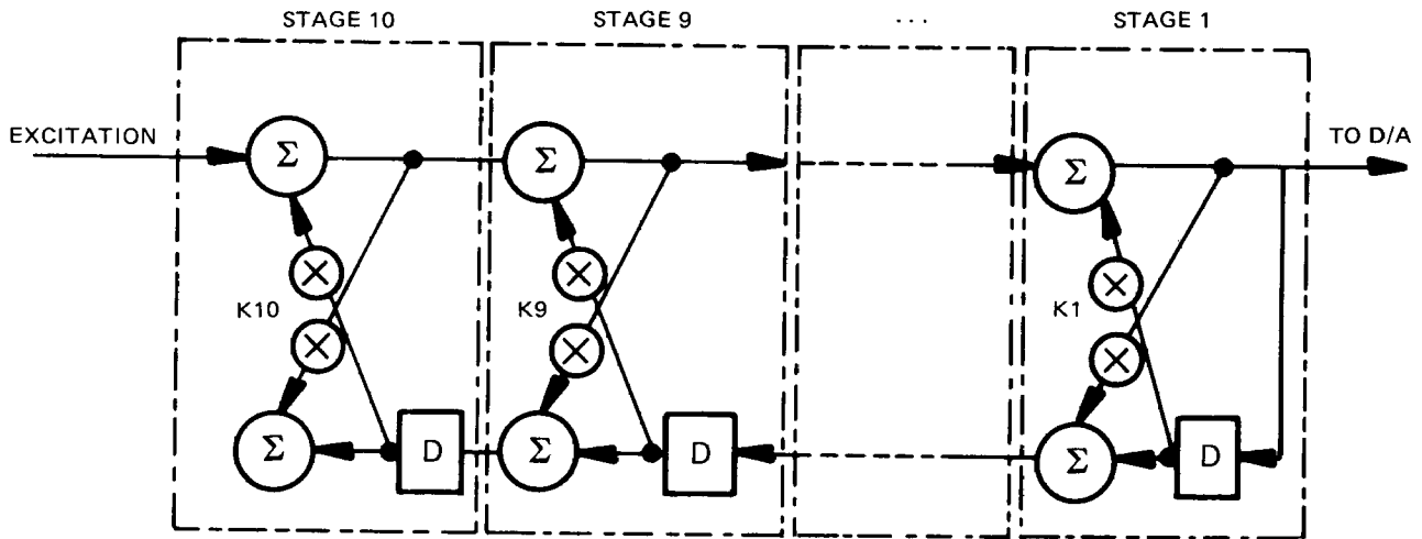
FIGURE 3 – TEN-STAGE DIGITAL LATTICE FILTER
