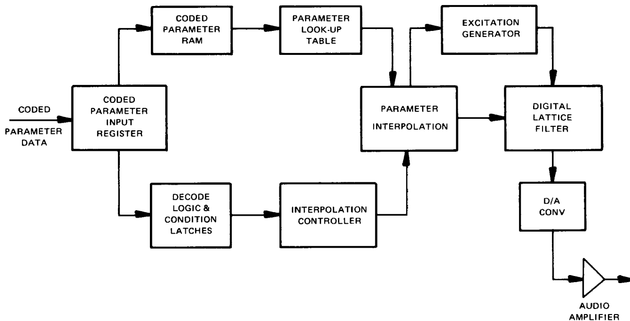
FIGURE 2 – SYNTHESIZER BLOCK DIAGRAM
