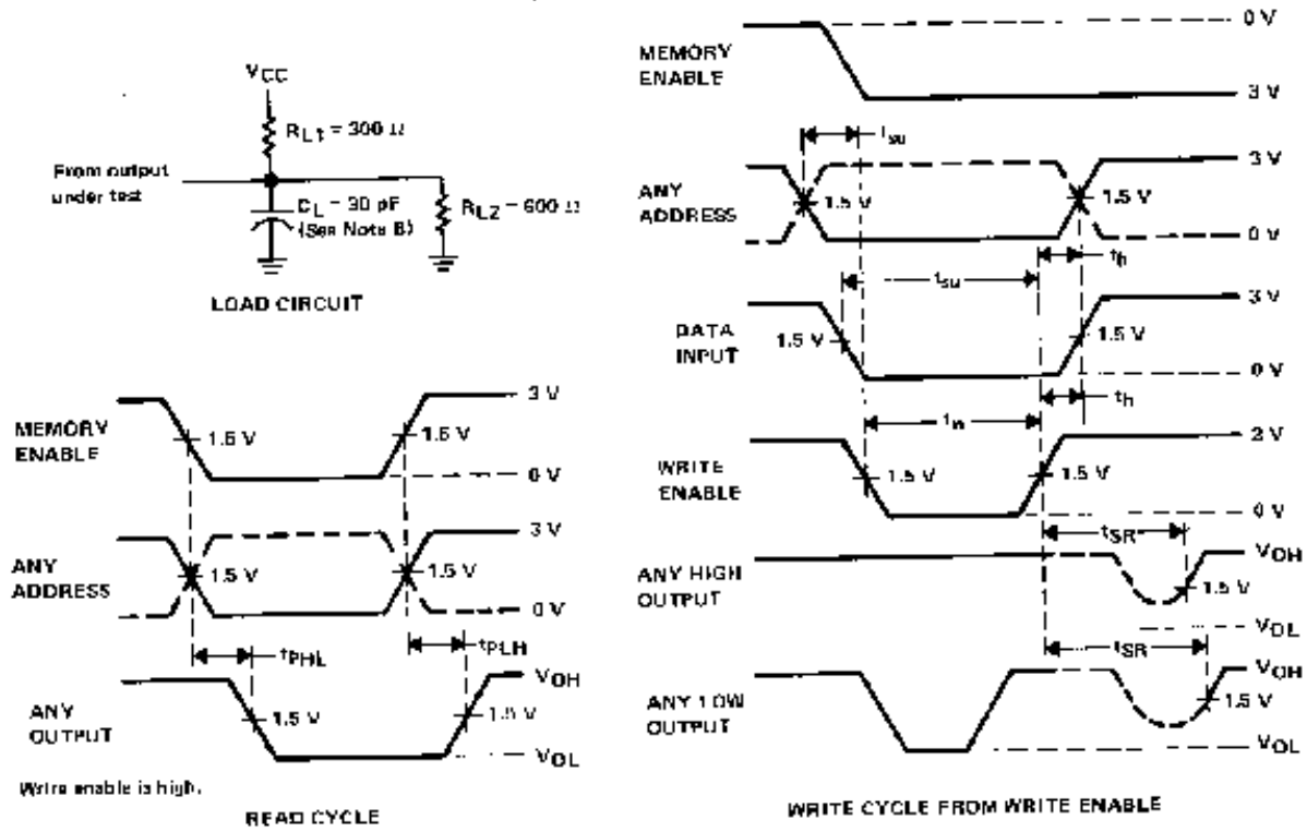
FIGURE 1 SWITCHING CHARACTERISTICS
