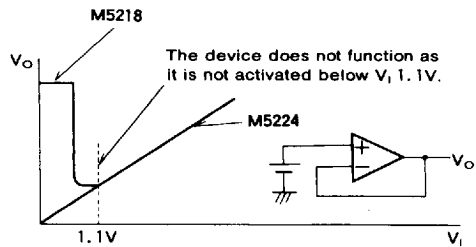
Single power supply operational amplifier M5224
