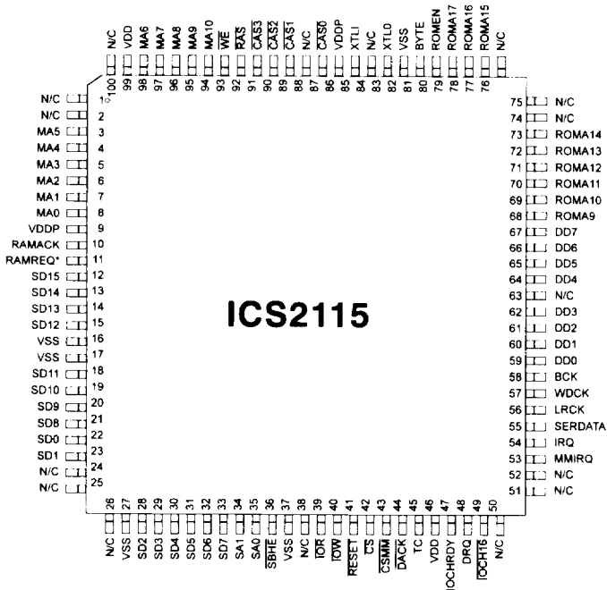
100-Pin TQFP, J-11
