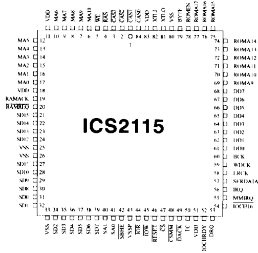
84-Pin PLCC, J-10
