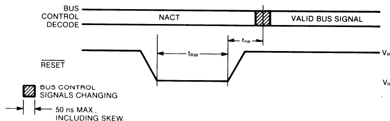
Fig. 8 RESET TIMING
