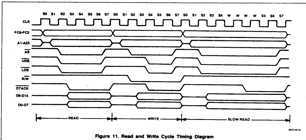
Figure 11. Read and Write Cycle Timing Diagram
