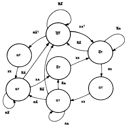
a. State Diagram for Mask Sets Previous to GN7
