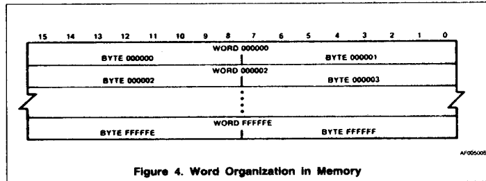
Figure 4. Word Organization in Memory
