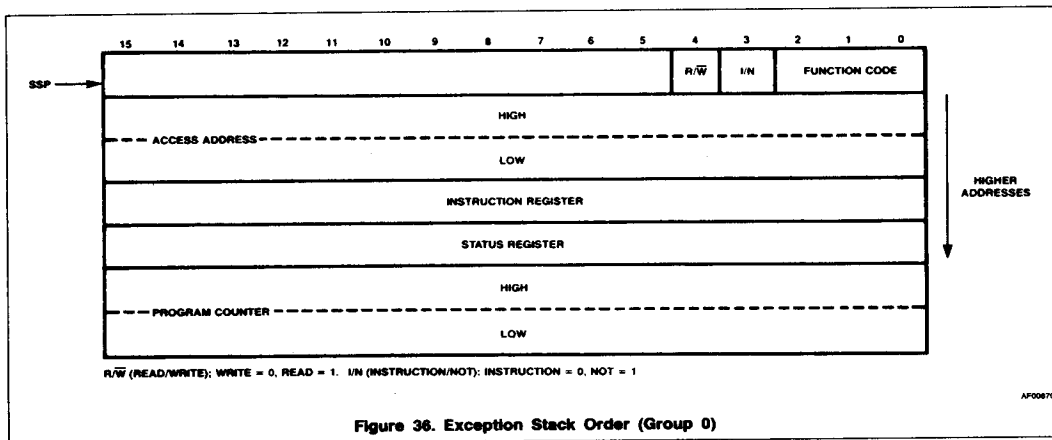
Figure 36. Exception Stack Order (Group 0)
