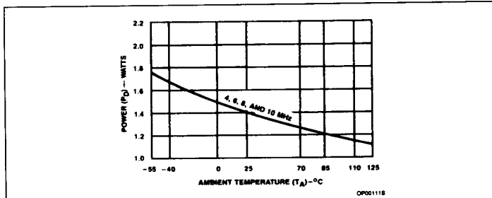
Figure 45. SCN68000 Power Dissipation ( P_D ) vs Ambient Temperature ( T_A )
