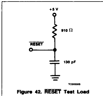
Figure 42. RESET Test Load
