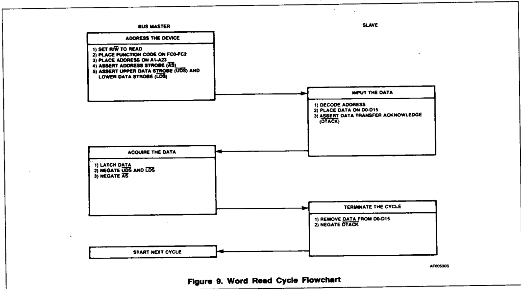
Figure 9. Word Read Cycle Flowchart
