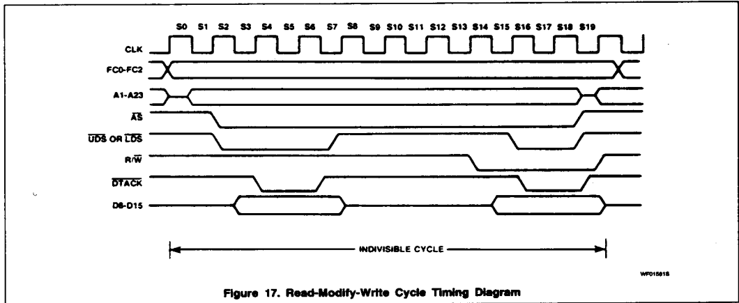
Figure 17. Read-Modify-Write Cycle Timing Diagram
