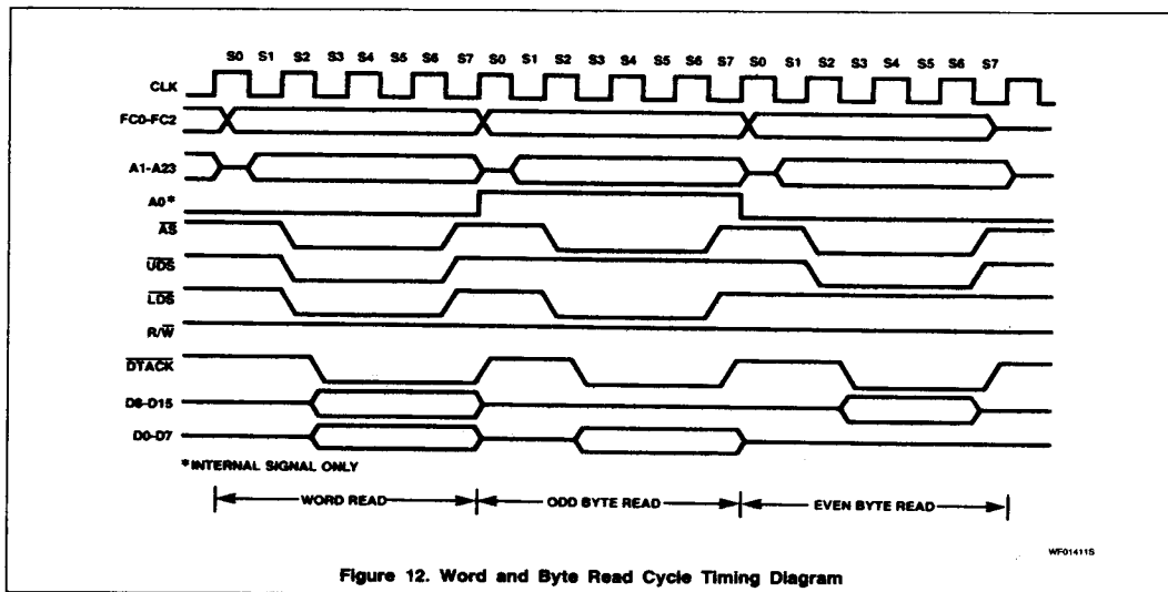
Figure 12. Word and Byte Read Cycle Timing Diagram
