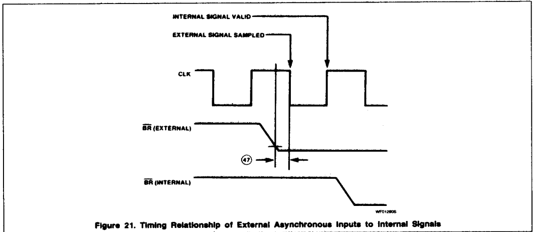
Figure 21. Timing Relationship of External Asynchronous Inputs to Internal Signals
