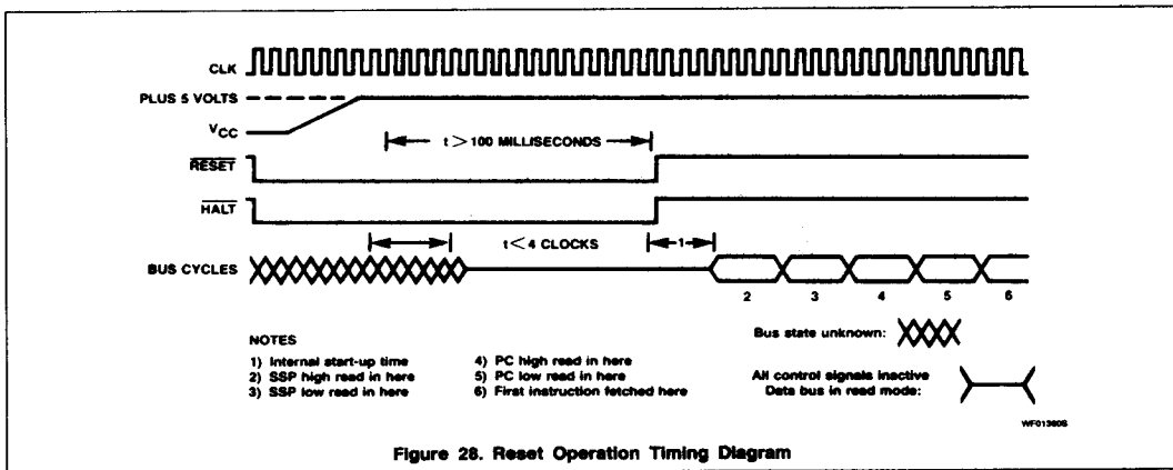
Figure 28. Reset Operation Timing Diagram
