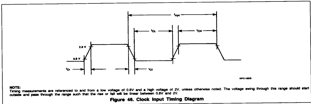
Figure 46. Clock Input Timing Diagram
