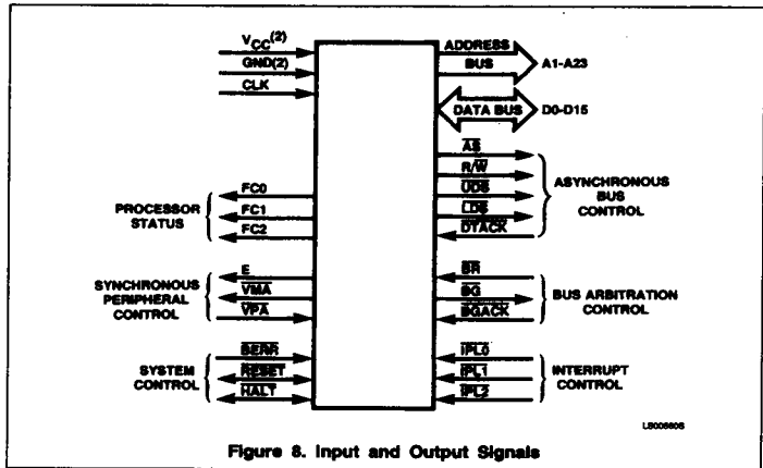
Figure 8. Input and Output Signals
