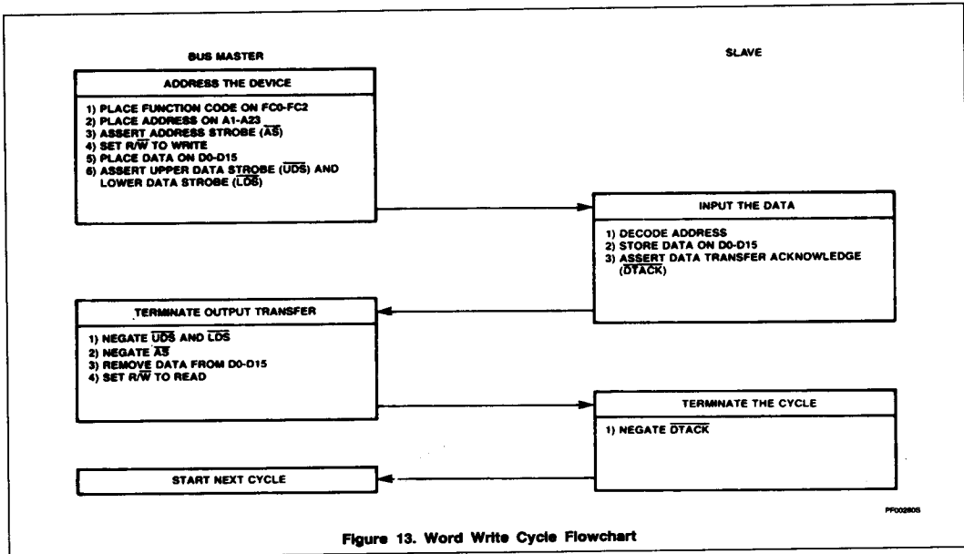
Figure 13. Word Write Cycle Flowchart
