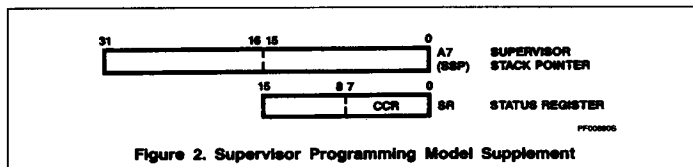
Figure 2. Supervisor Programming Model Supplement
