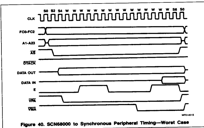
Figure 40. SCN68000 to Synchronous Peripheral Timing—Worst Case
