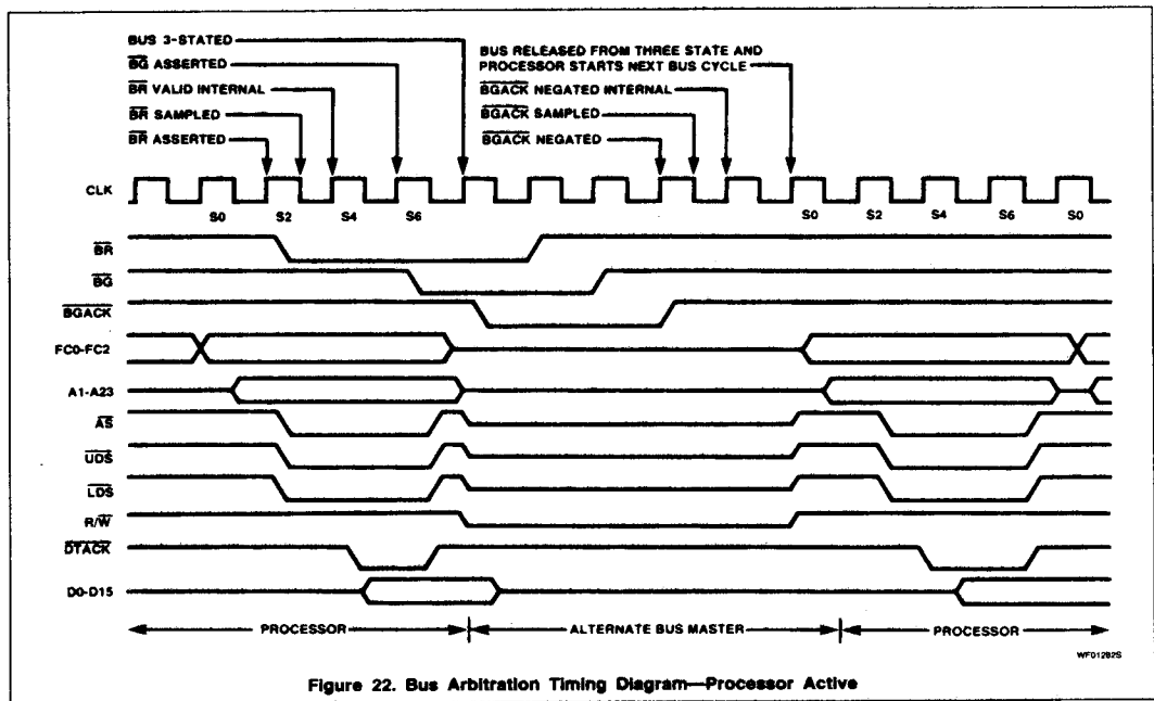
Figure 22. Bus Arbitration Timing Diagram—Processor Active
