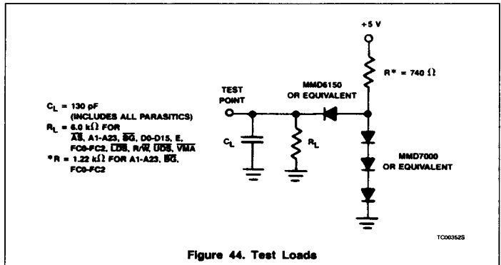
Figure 44. Test Loads
