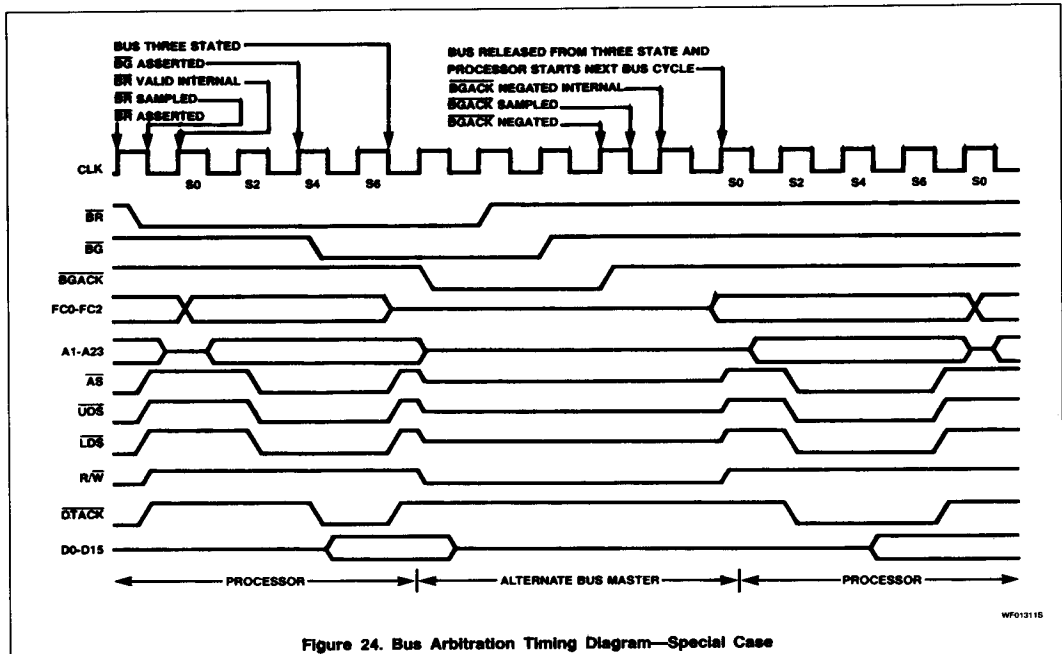
Figure 24. Bus Arbitration Timing Diagram—Special Case
