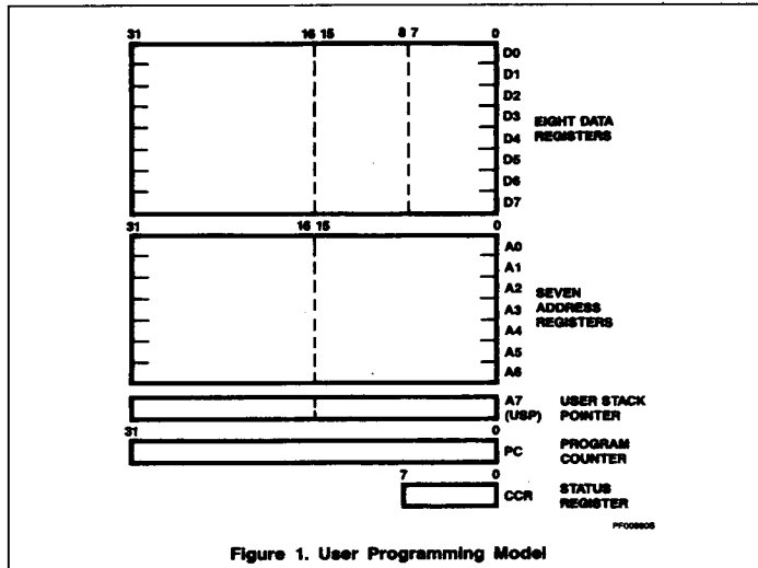
Figure 1. User Programming Model
