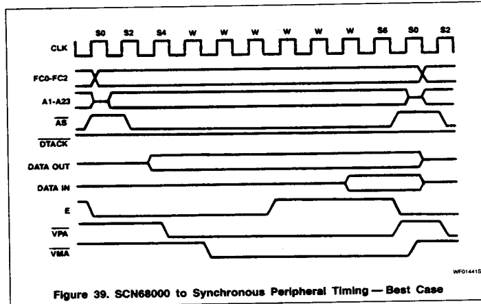
Figure 39. SCN68000 to Synchronous Peripheral Timing — Best Case
