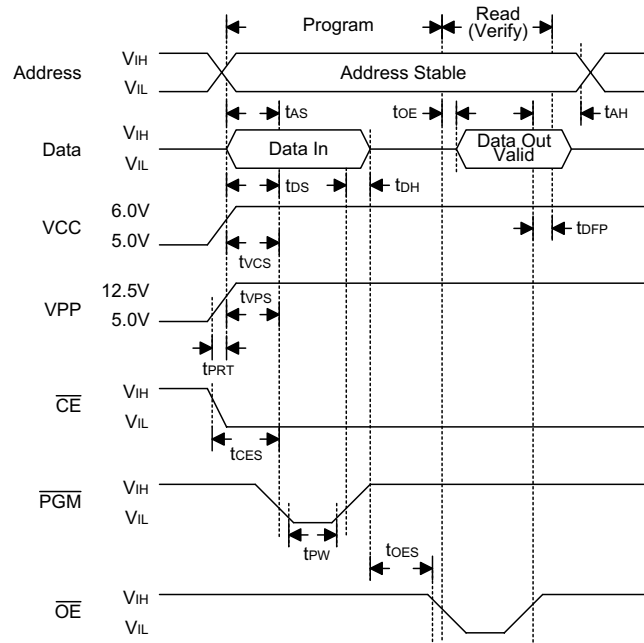
Figure 2. Programming waveforms
