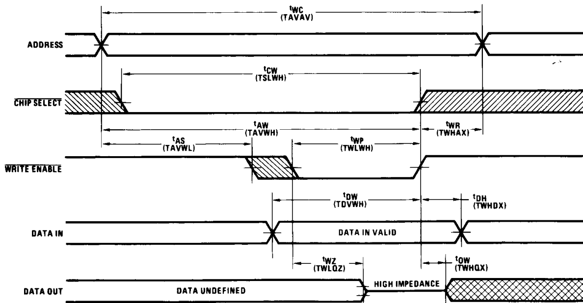
Write Cycle 1 (Write Enable Limited)
